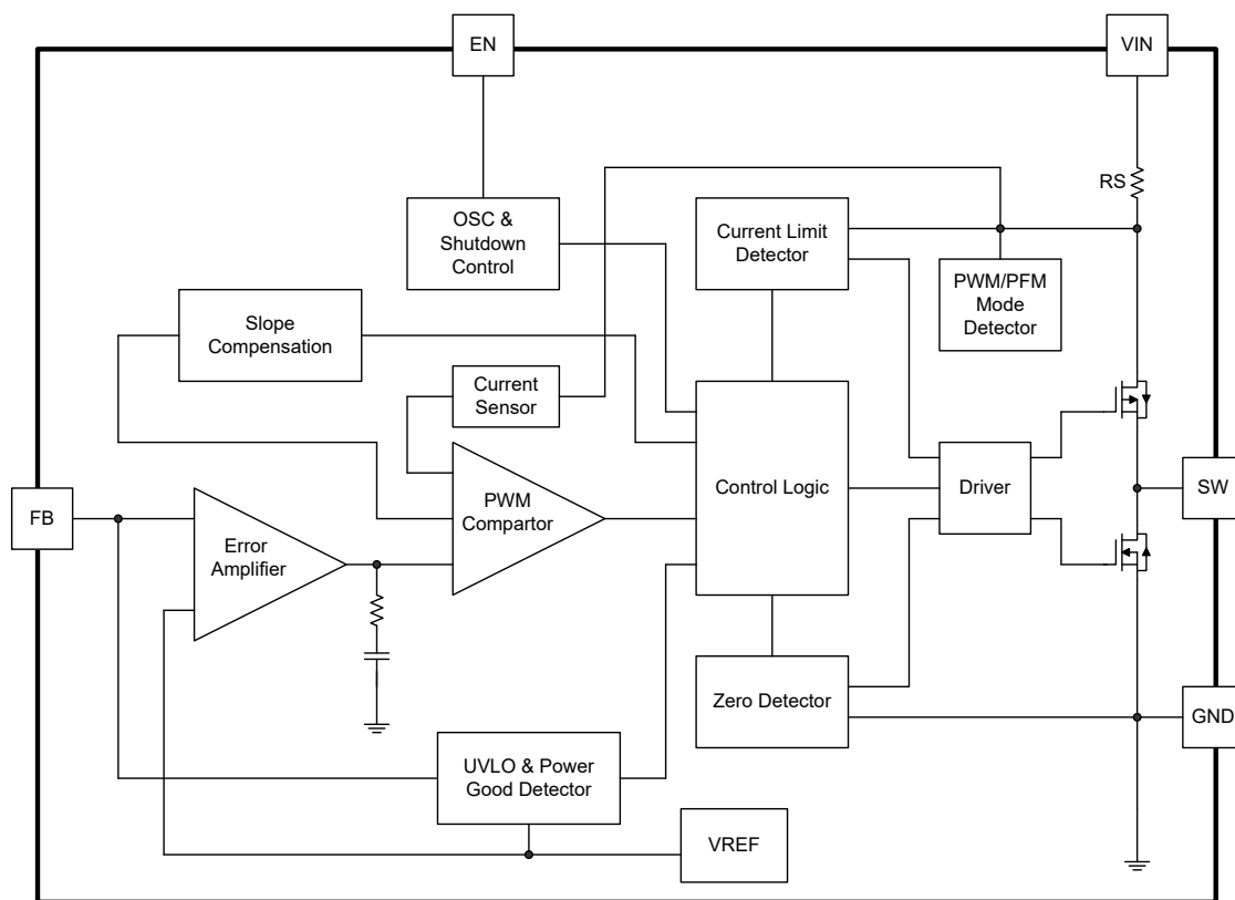
Block Diagram
