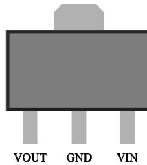
SOT89B (TOP view)
