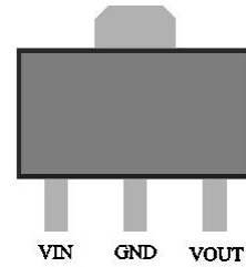
SOT89C(TOP view)
